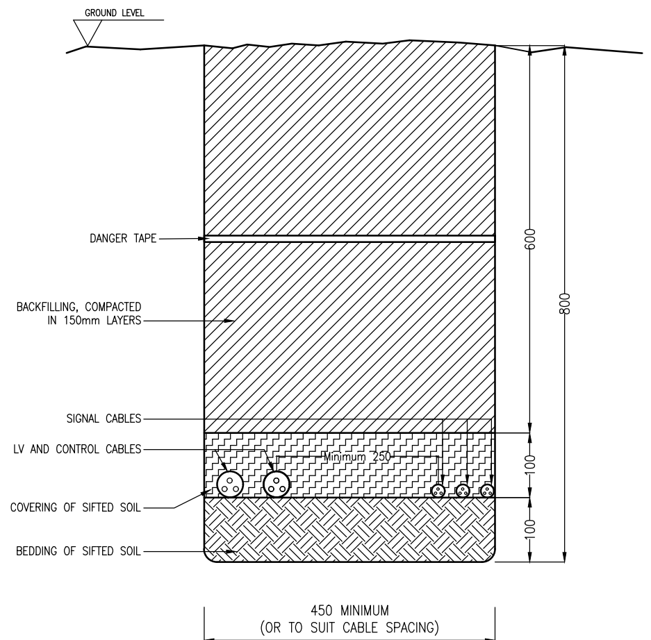
COMBINED LV, CONTROL AND SIGNAL CABLE TRENCH
