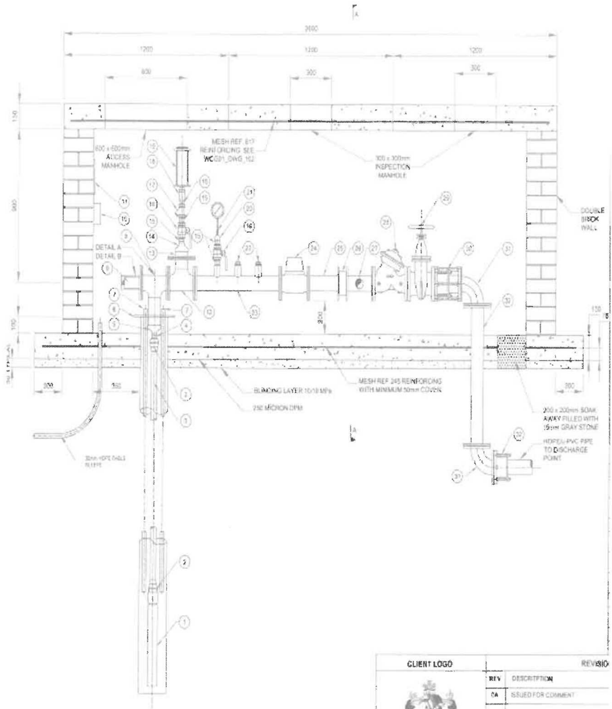
SECTION B-B
